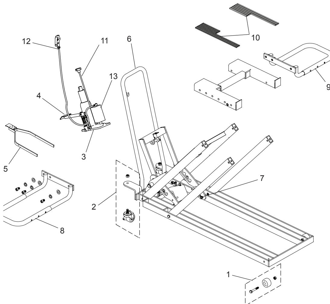
Figure 5 - Replacement Parts Illustration for Model T-5501
