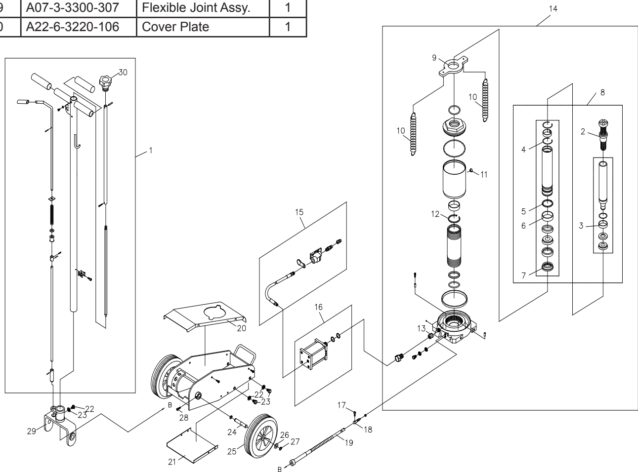
Figure 2 - Replacement Parts Illustration for Model 23227
