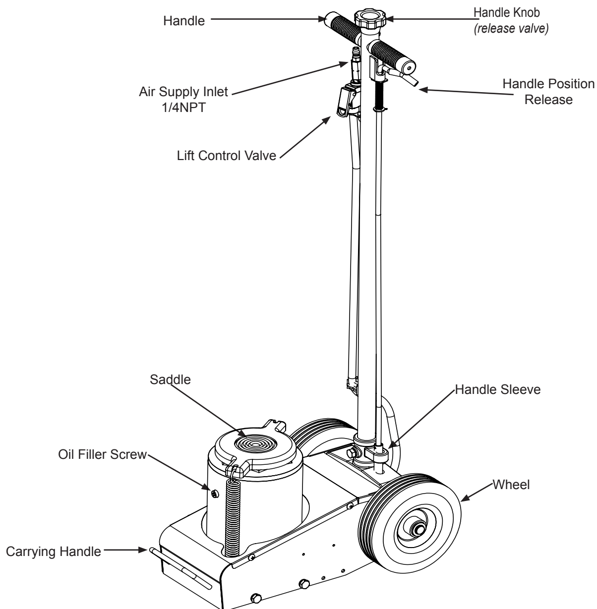
Figure 1 - Typical Truck Jack Nomenclature (23227 shown)
